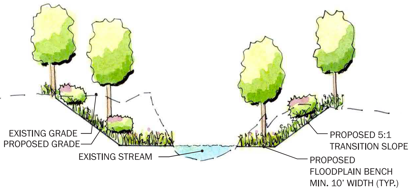
Typical Section
